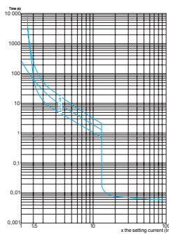
Kioldási jelleggörbe / Tripping characteristic
