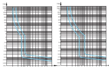
B karakterisztika / Characteristic B
