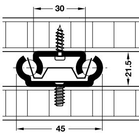
Mounted as shelf runner
