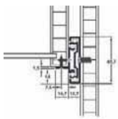
Bottom mounted
