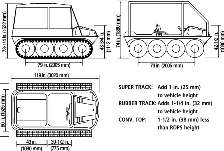
Vehicle shown with accessories, see specification page for base vehicle. (ARGO 8x8 750 HDi model shown)
